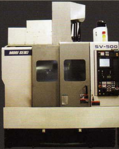
Frees Machine's Mori Seiki SV-500 BT-50 X = 960mm Y = 480mm Z = 520mm
