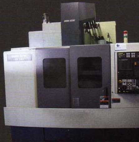
Frees Machine's Mori Seiki SV-500 BT-50 X = 960mm Y = 480mm Z = 520mm
